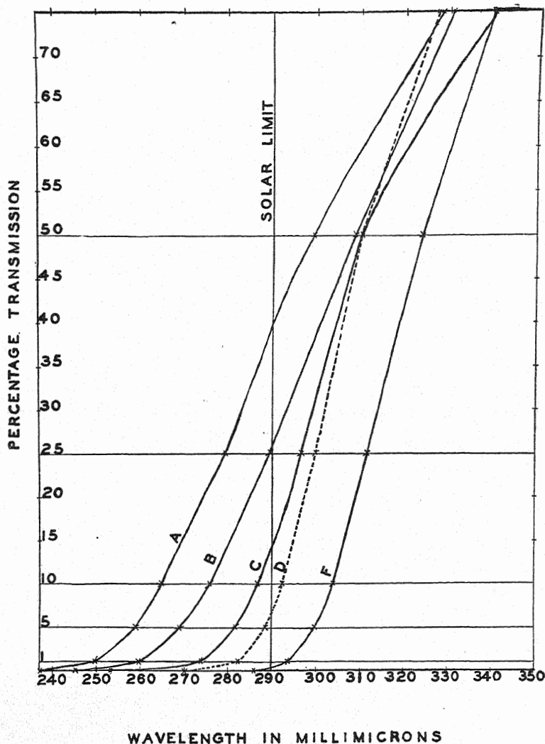
TEXT FIG. 2. Transmission graphs of various filters.
