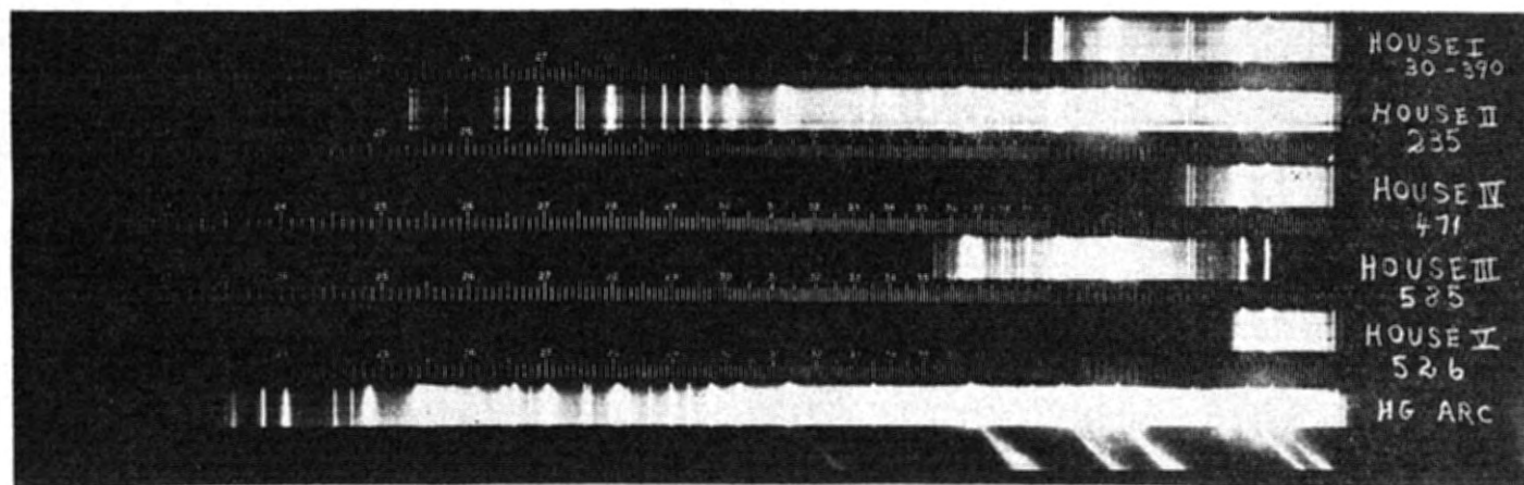
TEXT FIG. 2. Transmission spectra of the glasses used. Spectra obtained by use of a Hilgar quartz spectrograph illuminated with a mercury-vapor arc in quartz. The figures on the scale show the wave length in hundredths of microns.
