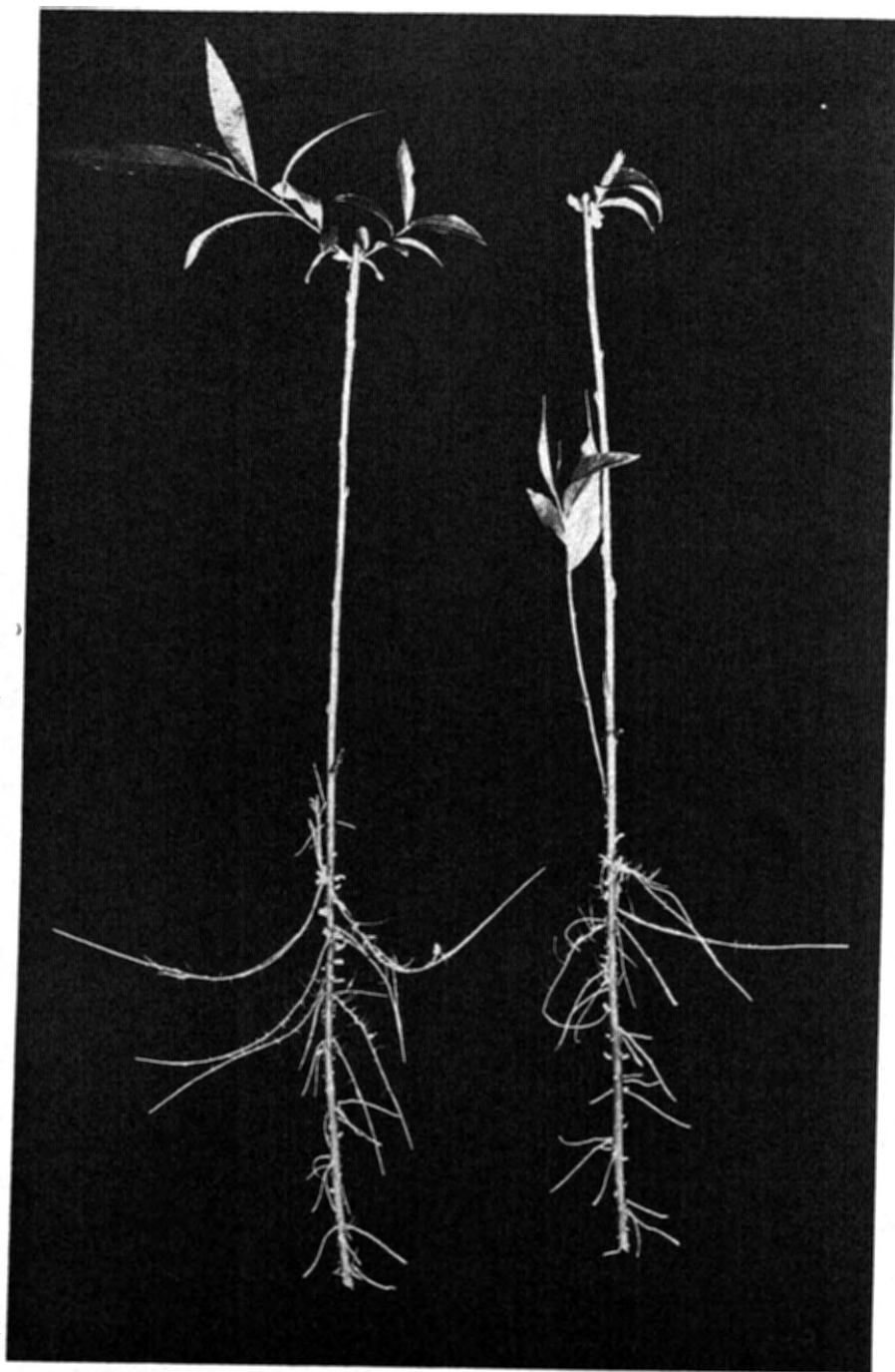
TEXT FIG. 5. Willow cutting in non-aerated water. Note the hypertrophied lenticels near the surface of the water and how they decrease in size to the base of the cutting where the oxygen supply was low (0.1 to 0.3 parts per million of water).
