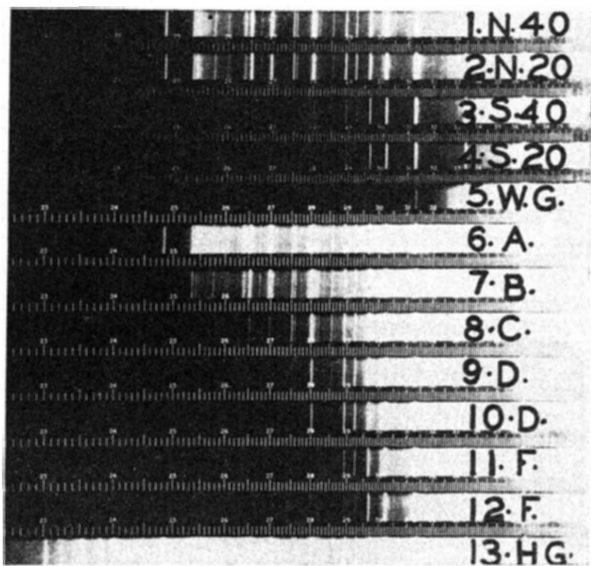
TEXT FIG. 1. Transmission spectra.
