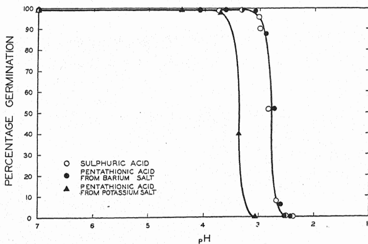
FIG. 8. The percentage of germination of conidia of Macrosporium sarcinaeforme in solutions of H_2SO_4 and H_2S_5O_6 plotted against the pH of these solutions.
