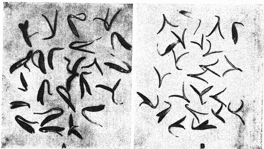
TEXT FIG. 5. Germination of embryos after four days when taken from seeds made partly dormant by covering with agar. A, a thin layer of agar in a petri dish; B, buried deeply in agar in a test tube.
