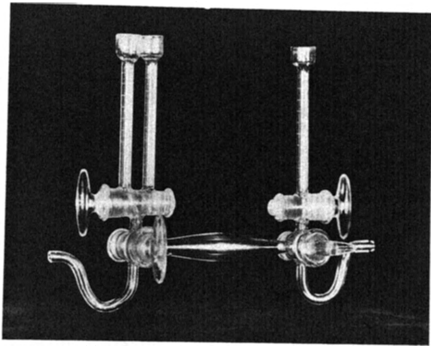
TEXT FIG. 1. Apparatus used for micro-determination of oxygen in water.
