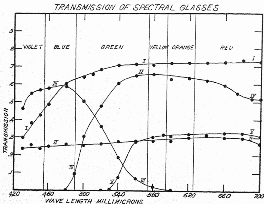
TEXT FIG. 1. Transmission curves for glass of spectral houses. The Correx, house II, was unpolished. Actually it transmits about 80 percent of the light instead of 25 percent. The measurements were made on a König-Martens spectrophotometer.
